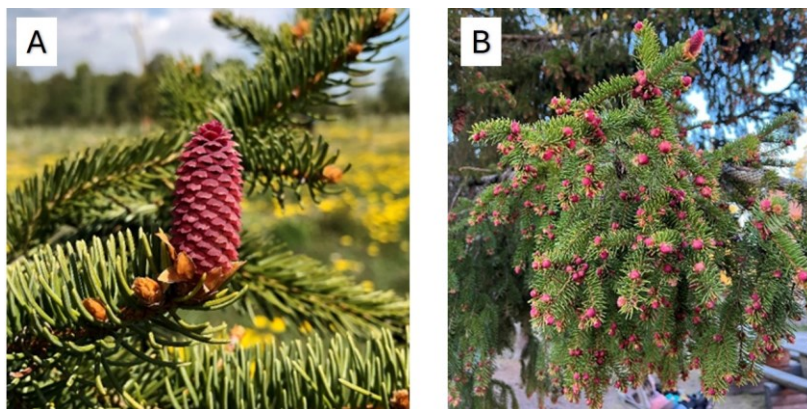
Figure 1. P. abies reproductive cones
