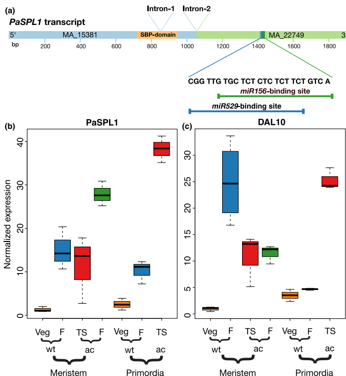
Fig. 3 Verification of expression of PaSPL1
