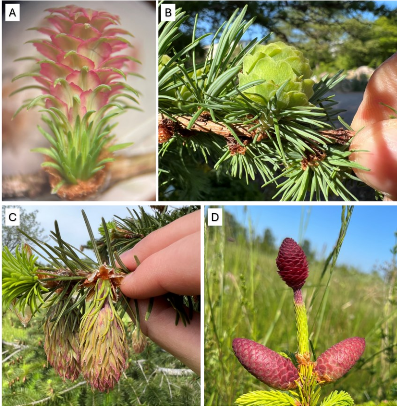
Figure 4. Larix cones, Pseudotsuga cones, and acrocona transition shoot
