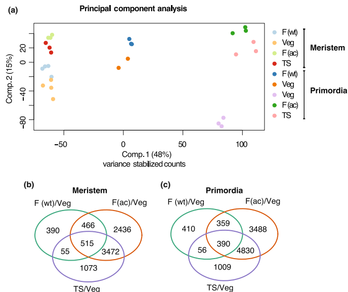
Fig. 2 Transcriptome sequencing of acrocona transition shoots. (a) Principal component analysis of RNA-sequencing data from 27 samples. The first and second principal components (PC1 and PC2) define the x- and y-axes of the two-dimensional space, respectively. PC1 represents 48%, and PC2 represents 15% of the total variation in the samples. Coloured dots represent wild-type and acrocona samples of different bud types, in bud meristem and primordia samples. F(ac), acrocona female sample; F(wt), wild-type female sample; TS, acrocona transition shoot sample; Veg, wild-type vegetative sample. (b) Venn diagram representing differentially expressed genes (DEGs) in meristem samples collected during the early growth phase in summer, whereas the Venn diagram in (c) shows the distribution of DEGs in primordia samples collected during the late growth phase in the autumn. The green circles represent DEGs between female wild-type samples and vegetative samples (F(wt)/Veg). The orange circles represent DEGs between female acrocona samples and vegetative samples (F(ac)/Veg). The violet circles represent DEGs between acrocona transition shoot samples and vegetative samples (TS/Veg). The threshold to judge the significance of gene expression differences was false discovery rate (FDR) \leq 0.01 and the absolute value of \log_2 FoldChange ( \log_2 FC) \geq 0.5 .
