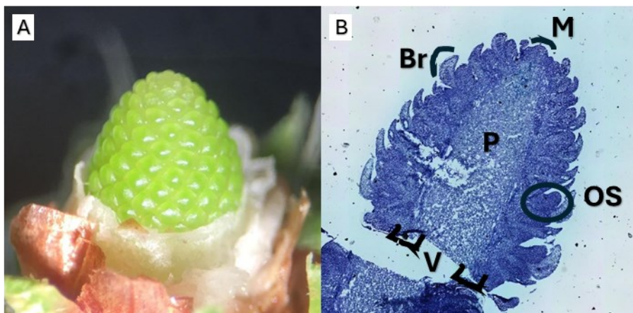
Figure 2. P. abies seed cone primordia in detail
