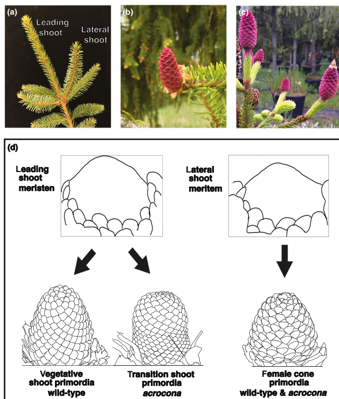
Fig. 1 Illustration of female cones, vegetative shoots and acrocona transition shoots.
