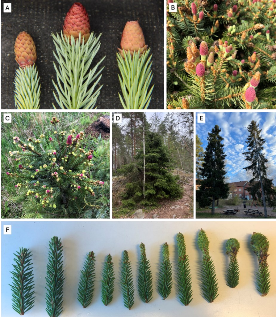
Figure 3. Picea reproductive mutants
